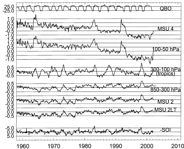
FIG. 2. The top and bottom traces are time series of the QBO ( \text{m s}^{-1} ) and normalized SOI (dimensionless), respectively. The QBO is represented by the 50-hPa zonal wind at Singapore. The SOI is based on Trenberth (1984). The other time series are multidataset-average monthly temperature anomalies for six different layers. All temperature time series are for the globe, except for the 300–100-hPa-layer time series, which is for the Tropics.
