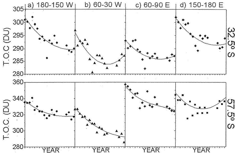
Figure 4. Evolution of annual TOC 1980–2000 for a selection of “bins” at (top) 32.5°S and (bottom) 57.5°S at (a) 180°–150°W, (b) 60°–30°W, (c) 60°–90°E, and (d) 150°–180°E. Symbols (circles, triangles, diamonds, and squares) show the mean of the observations for each bin, and the curves show the result of the cubic polynomial fit of those points.
