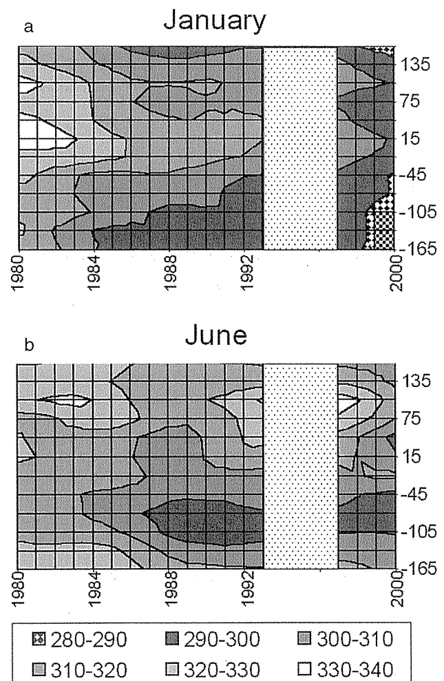
Figure 6. TOC evolution between 1980 and 2000 during (a) January and (b) June at 47.5°S.
