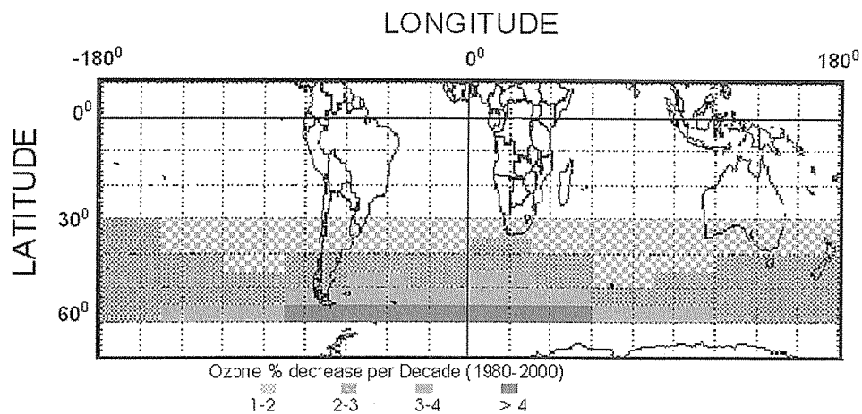
Figure 1. TOC 20-year linear trend evolution between 30° and 60°S. A distinct dependence on both longitude and latitude can be observed for the trends.
