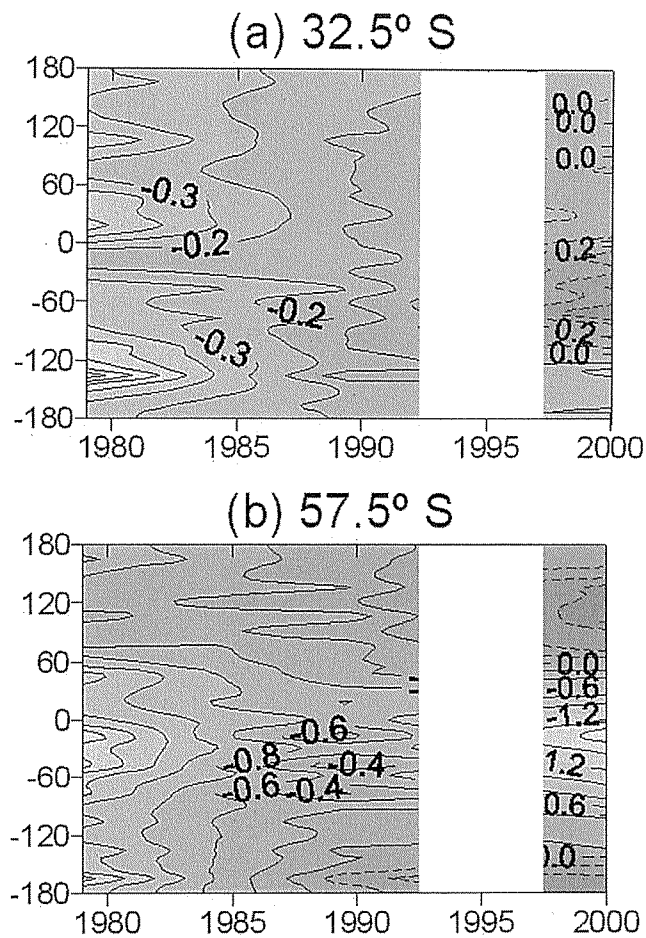
Figure 5. Longitude-time variations for the smoothed annual trend estimate, derived from the cubic polynomial fit, at (a) 32.5°S and (b) 57.5°S. Annual trend is given as a percentage change from the previous year's TOC.
