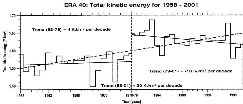
Figure 5. Total kinetic energy, K , annually averaged, calculated from ERA40 for the period 1958–2001. Figure 5 is in two parts, the first showing the years 1958–1978, the second part showing the years 1979–2001. A trend line is indicated for the whole period as well as separately for the two periods. See color version of this figure in the HTML.
