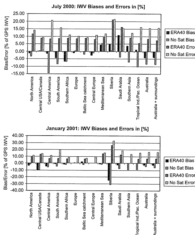
Figure 4. IWV bias and total error for (top) July 2000 and (bottom) January 2001 from comparison with GPS measurements in selected areas (see Table 4). Darker shaded vertical bars indicate the results from ERA40; lighter shaded bars indicate results from the NOSAT experiment. Note the dry bias, particularly in the NOSAT experiment.
