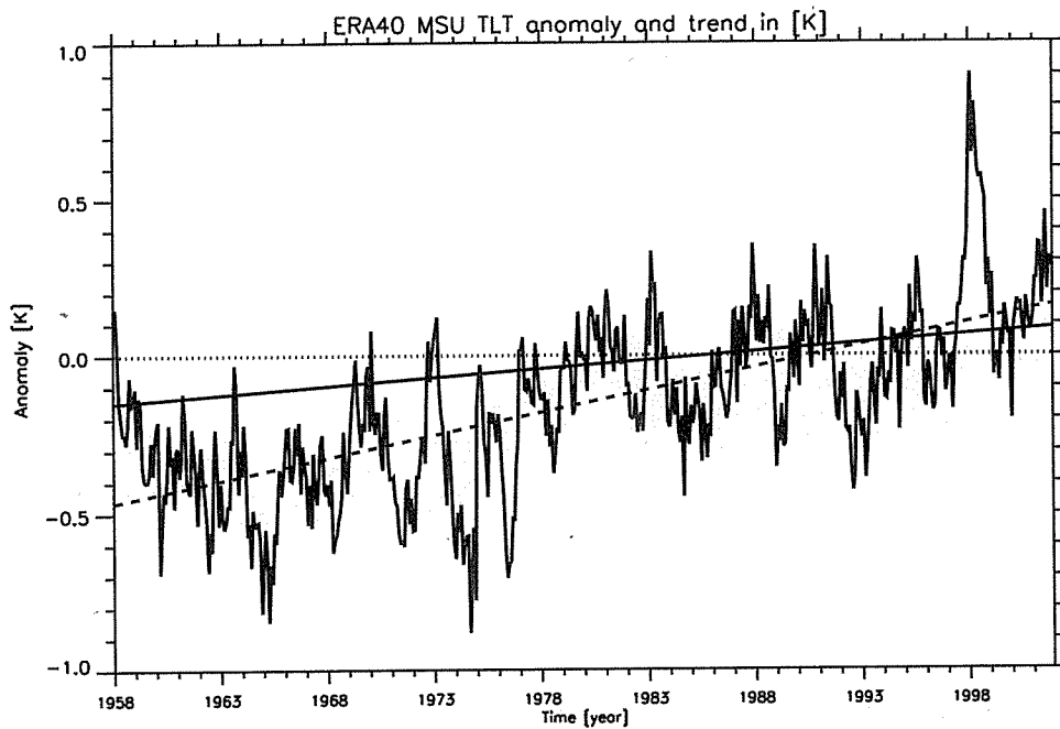
Figure 2. TLT calculated from ERA40 for the period 1958–2001. The dashed line shows the corresponding warming trend. The full line indicates a corrected warming trend obtained by adding a factor to the data for the period 1958–1972 obtained from the difference between ERA40 and the NOSAT experiment, and by excluding data for the years 1972–1978. See color version of this figure in the HTML.
