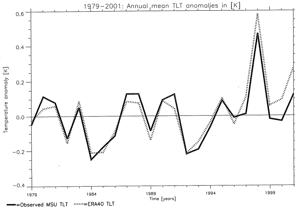
Figure 1. Lower tropospheric temperature, TLT, from MSU measurements (solid line) and calculated from ERA40 (dashed) for the period 1979–2001.
