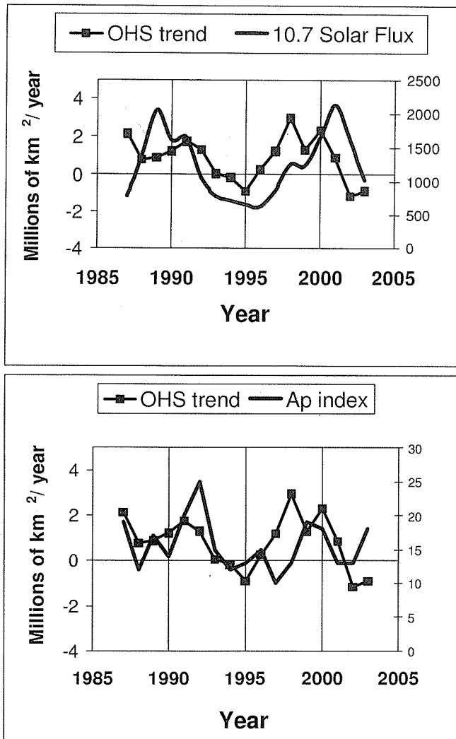
Figure 3. Changes in the slopes of 6-year subsets of the monthly average OHS data compared to the monthly means of the 10.7-cm solar flux index and the geomagnetic A_p index during the month of September.
