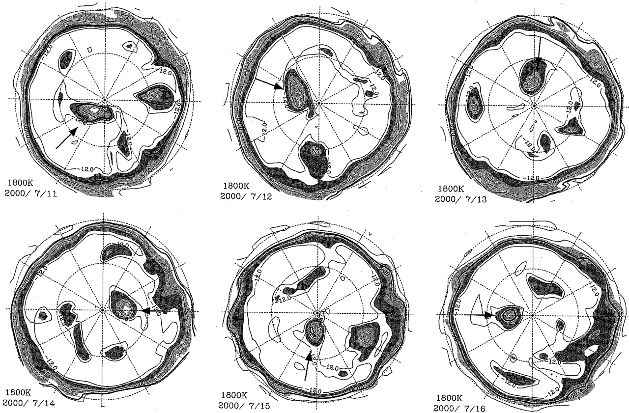
Figure 5. Time evolution of PV field on 1800 K isentropic surface in 2000. The maps are Lambert equal area projections, with the dashed lines of 30°S and 60°S latitude circles. Thick lines are the polar vortex edge defined as the isoline of PV where the gradient of PV is largest in the equivalent latitude coordinate. 1 unit represents 10^{-3} \text{ Km}^2 \text{ s}^{-1} \text{ kg}^{-1} . Light-shaded is the region of PV from 4.5 to 7.5, and heavy-shaded is from 7.5 to 10.5.
