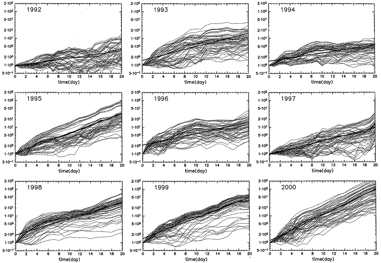
Figure 12. Time evolution of the contour length relative to the initial length. Contours initially put between 70°S and 80°S in Figure 11 are plotted in this figure. Thick lines are mean length of the contours. These are fitted to the thick straight lines.
