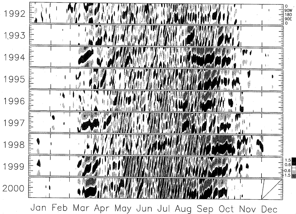
Figure 1. Time-longitude sections of the wavenumber 1 component of PV along 72^{\circ}\text{S} on 1800 K isentropic surface (approximately 1hPa). 1 unit represents 10^{-3} \text{ Km}^2 \text{ s}^{-1} \text{ kg}^{-1} . The lines of constant phase in the section of Dec 2000 are those for the periods of 4 days and 30 days.
