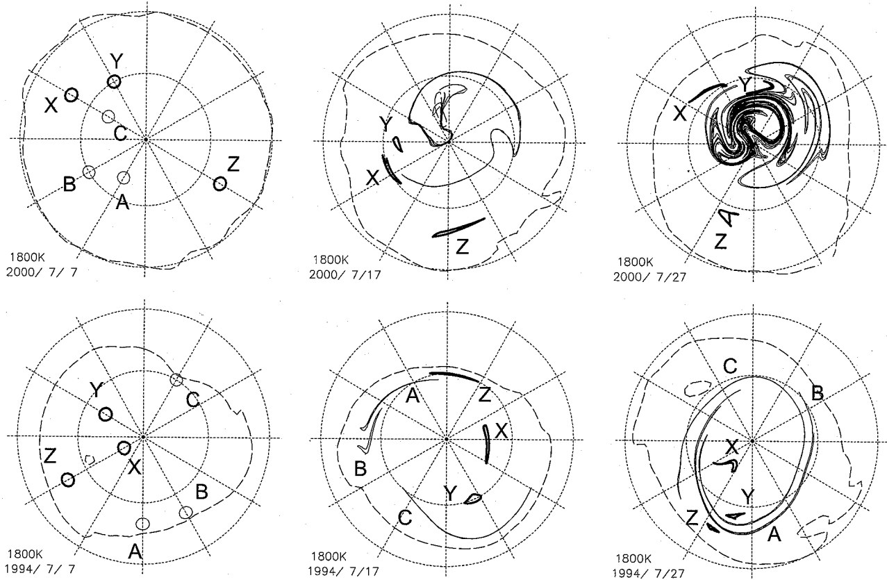
Figure 9. Advections of the six material contours. Thin contours (ABC) are the three longest ones after the 20-day advection. Thick contours (XYZ) are the three shortest ones. Initial positions of all the contours are shown in Figure 11.
