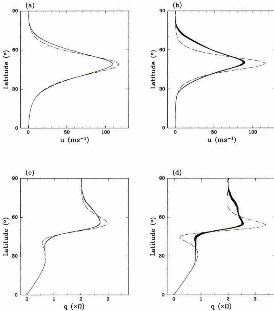
FIG. 1. Zonal mean zonal wind \bar{u}(\phi) and zonal mean PV \bar{q}(\phi) as a function of latitude for (a) and (c) the vacillation and for (b) and (d) the irregular solution. The profiles at every 1/5 vacillation cycle are drawn for the vacillation and at each day of 20 days for the irregular solution. The dashed lines are the prescribed \bar{u}_0(\phi) and \bar{q}_0(\phi) .
